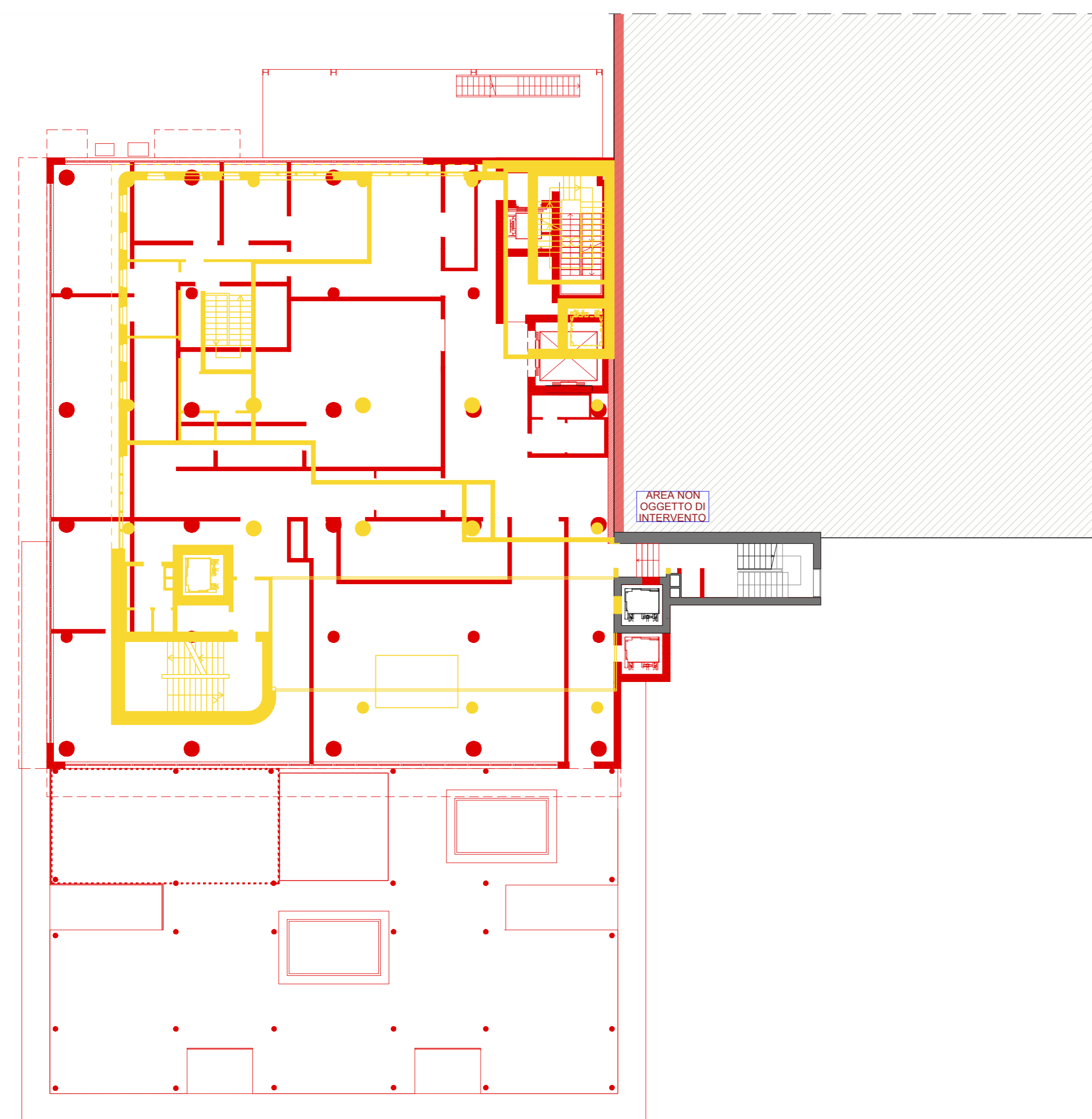
PIANTA PIANO PRIMO, +4.10, SG LAB (CLEAN ROOM)
